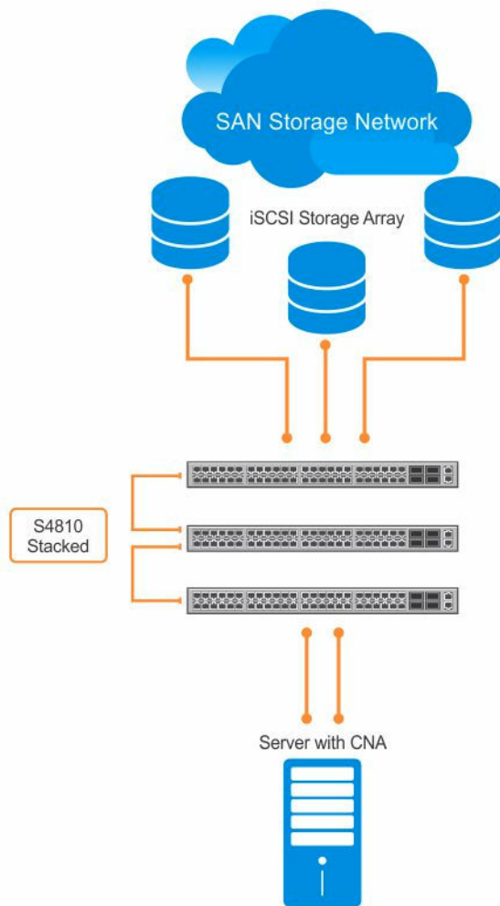
Figure 50. iSCSI Optimization Example
